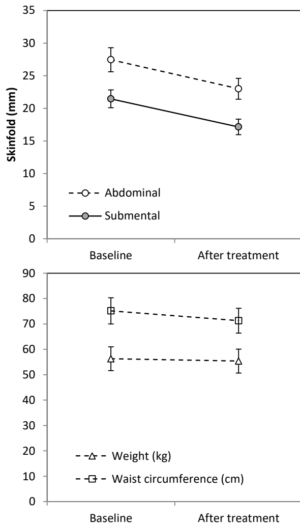
Fig 1: A) Skinfold thickness at baseline and after 3–6 sessions of combined Nd:YAG and Er:YAG laser treatment. Mean \pm SD of 11 patients with abdominal fat (open symbols) and 20 patients with submental fat (grey symbols) treated. B) Weight and waist circumference at baseline and after laser treatment for patients in the abdominal group only (mean \pm SD, n=11).
