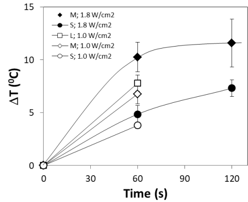
Fig. 4.: Measured temperature increases as a function of irradiation time ( t_{irr} ) during stamping PLLT for different spot size MarcCo™ handpieces and spot power densities ( P_s ). It should be noted that when using recommended PLLT protocols (See Tables 1 and 2) the resulting temperature increase is below 3°C.
